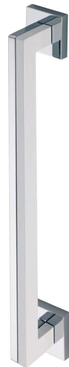
Model : E- 8001 Finish : CP-BSN, CP-Matt Black, CP-White Size : 250mm, 350mm Make : Zamak Applicable for : Glass, Wooden Doors
